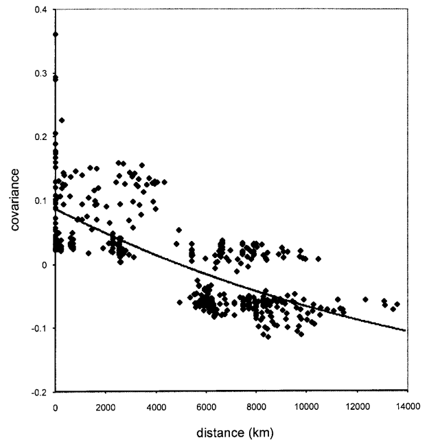
Figure 6 Relationship between geographic and genetic distance. Great circle distances (in kilometers) are plotted against the covariance of allele frequencies for 31 populations. A nonlinear regression line based on a one-dimensional Malécot model is fit to the data.
