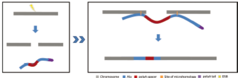
■ Chromosome ■ Alu ■ polyA spacer ■ Site of microhomology ■ polyA tail ■ DSB
